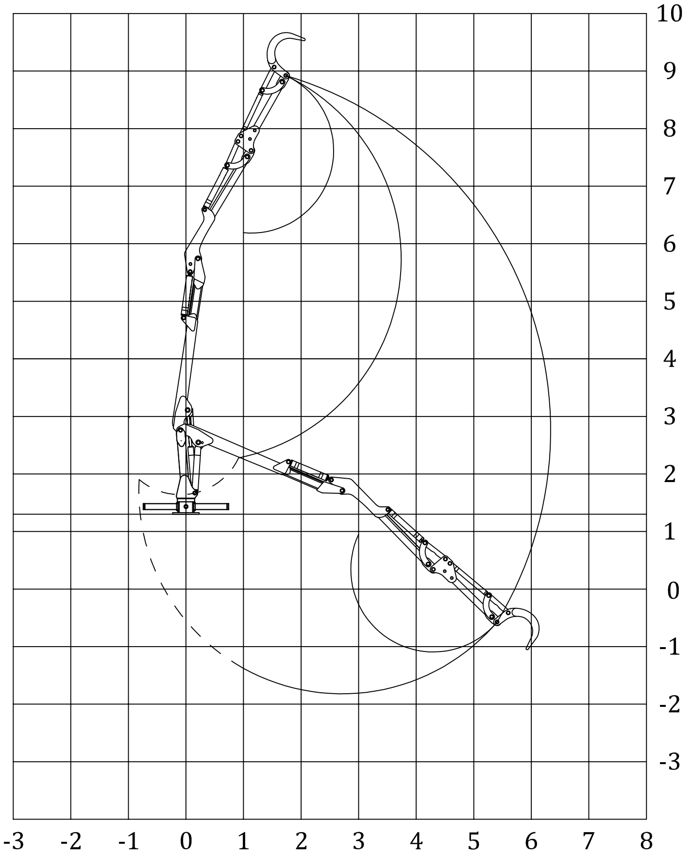
LIFTING DIAGRAM FOR UNLOADER RADIAL LOADER (All dimensions are in metres.)
